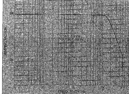
DAMPING FACTOR vs FREQUENCY
